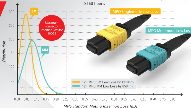
SENKO Low Loss 12F MPO Connectors - Made for 100GE and beyond 2160 fibers
